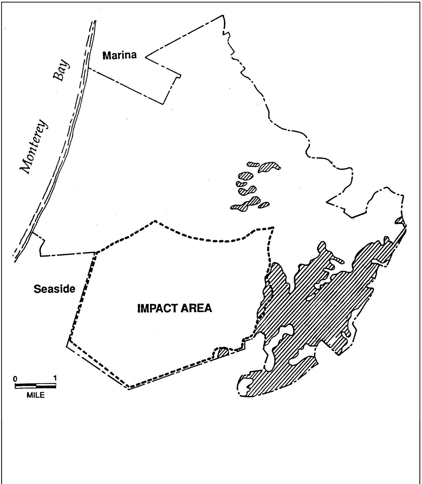
Figure 4.3-5 Soils with High Shrink-Swell Potential at Fort Ord
